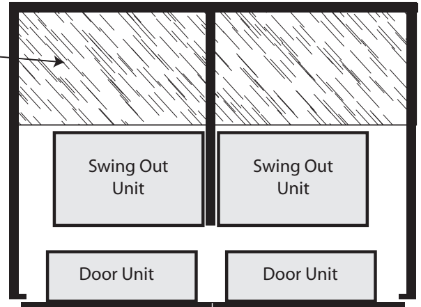
Top View Completed Installation
